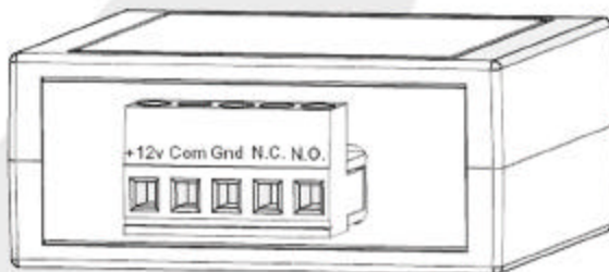
Power connections, VDC output and contact closures
